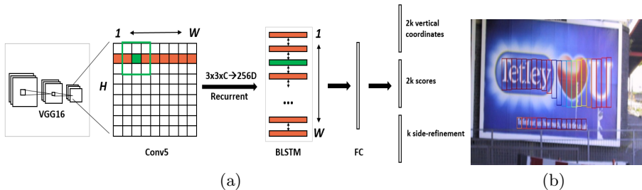
Fig. 1: (a) Architecture of the Connectionist Text Proposal Network (CTPN). We densely slide a 3 \times 3 spatial window through the last convolutional maps ( conv5 ) of the VGG16 model [27]. The sequential windows in each row are recurrently connected by a Bi-directional LSTM (BLSTM) [7], where the convolutional feature ( 3 \times 3 \times C ) of each window is used as input of the 256D BLSTM (including two 128D LSTMs). The RNN layer is connected to a 512D fully-connected layer, followed by the output layer, which jointly predicts text/non-text scores, y -axis coordinates and side-refinement offsets of k anchors. (b) The CTPN outputs sequential fixed-width fine-scale text proposals. Color of each box indicates the text/non-text score. Only the boxes with positive scores are presented.
